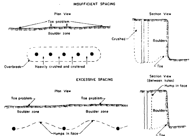
Figure 72.—Effects of insufficient and excessive spacing.
