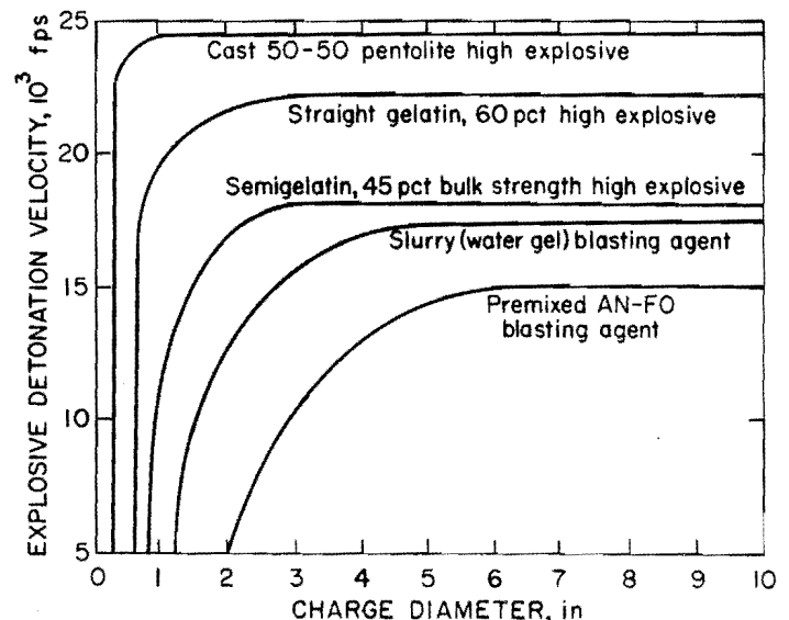
Figure 13.—Effect of charge diameter on detonation velocity.
