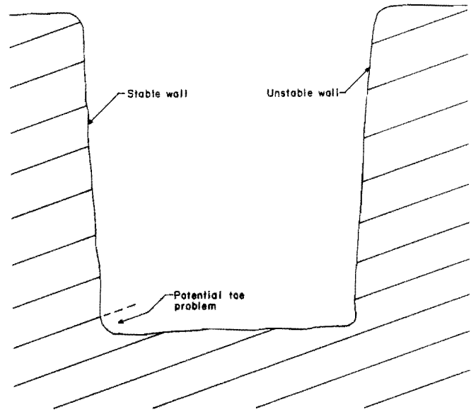
Figure 64.—Effect of dipping beds on slope stability and potential toe problems.
