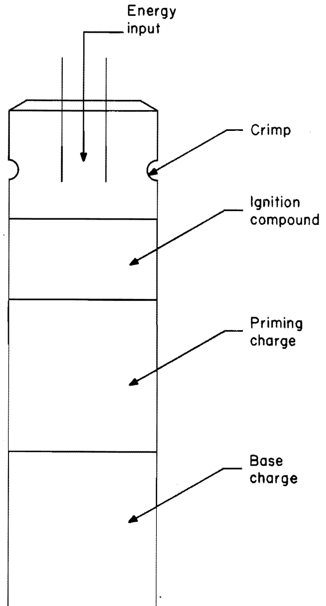
Figure 17.—Instantaneous detonator.
