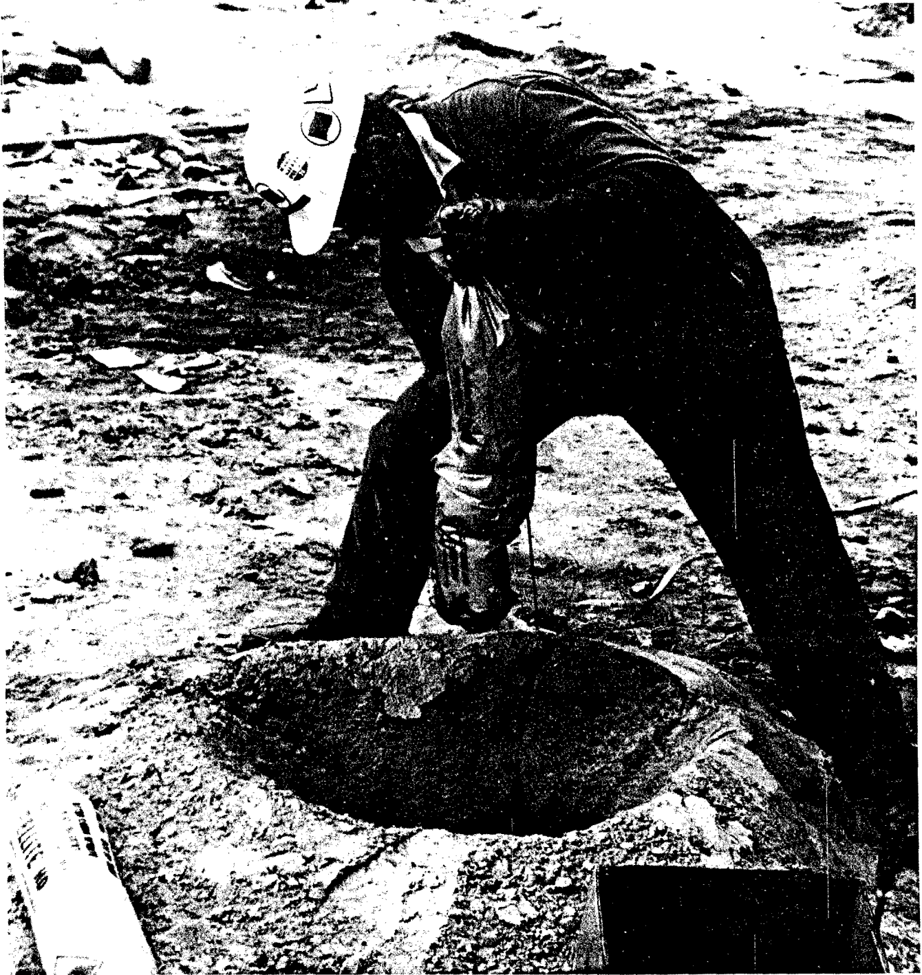
Figure 10.—Loading slurry-filled polyethylene bags. (Courtesy Atlas Powder Co.)
