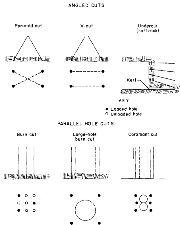
Figure 76.—Types of opening cuts.
