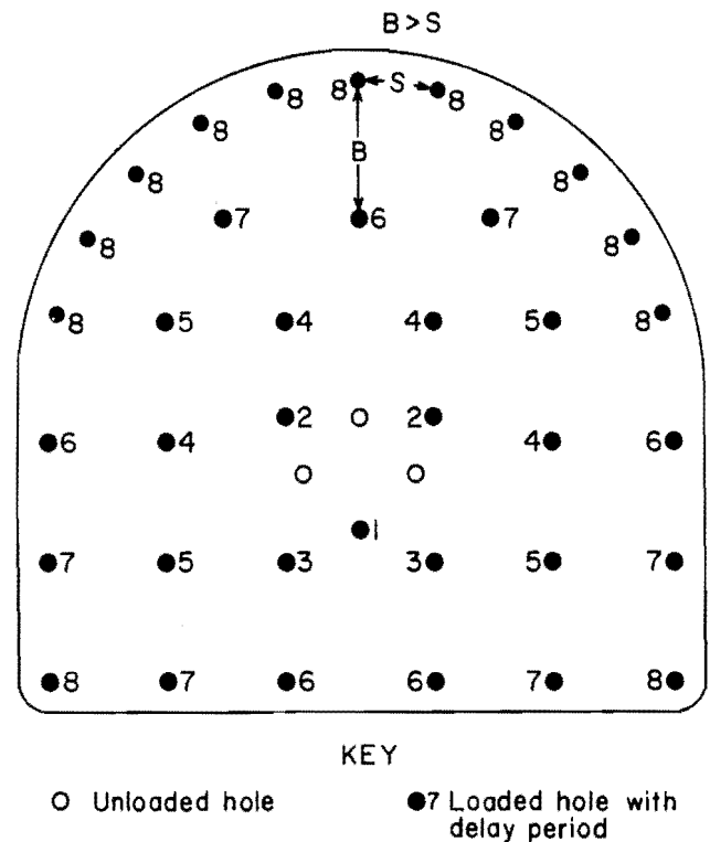
Figure 91.—Typical smooth blasting pattern (burden, B, is larger than spacing, S).
