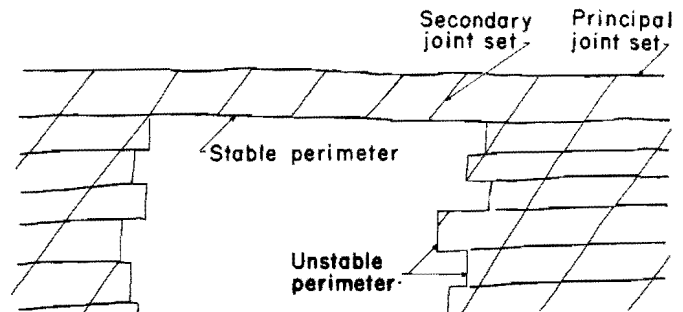
Figure 60.—Effect of jointing on the stability of an excavation.
