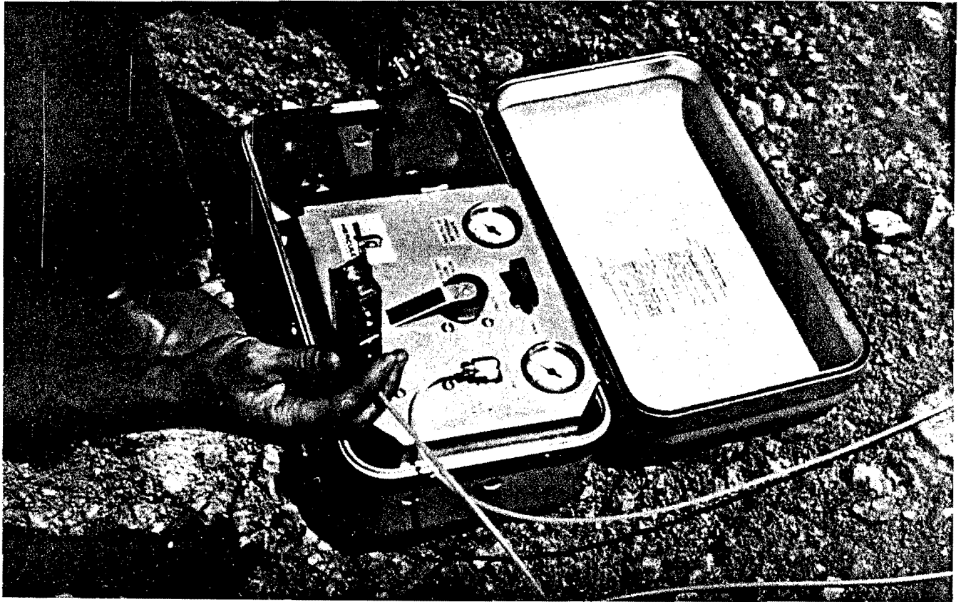
Figure 40.—Hercudet pressure test module. (Courtesy Hercules Inc.)
