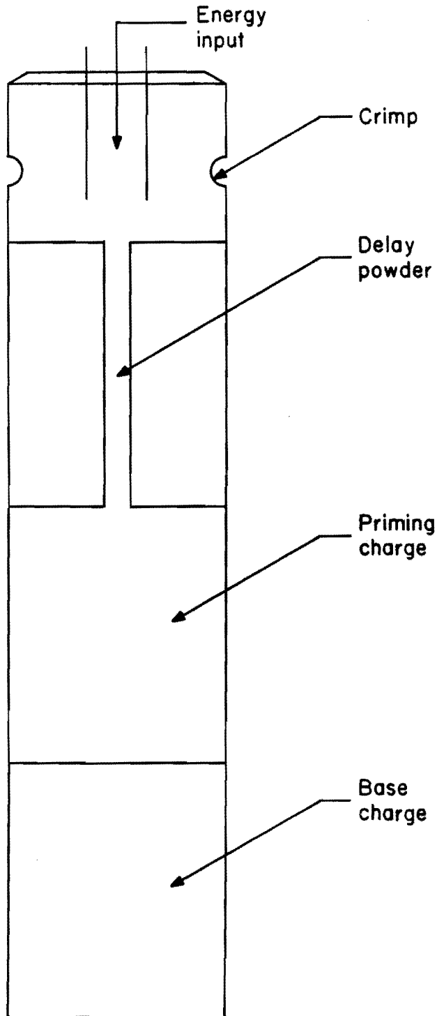
Figure 18.—Delay detonator.
