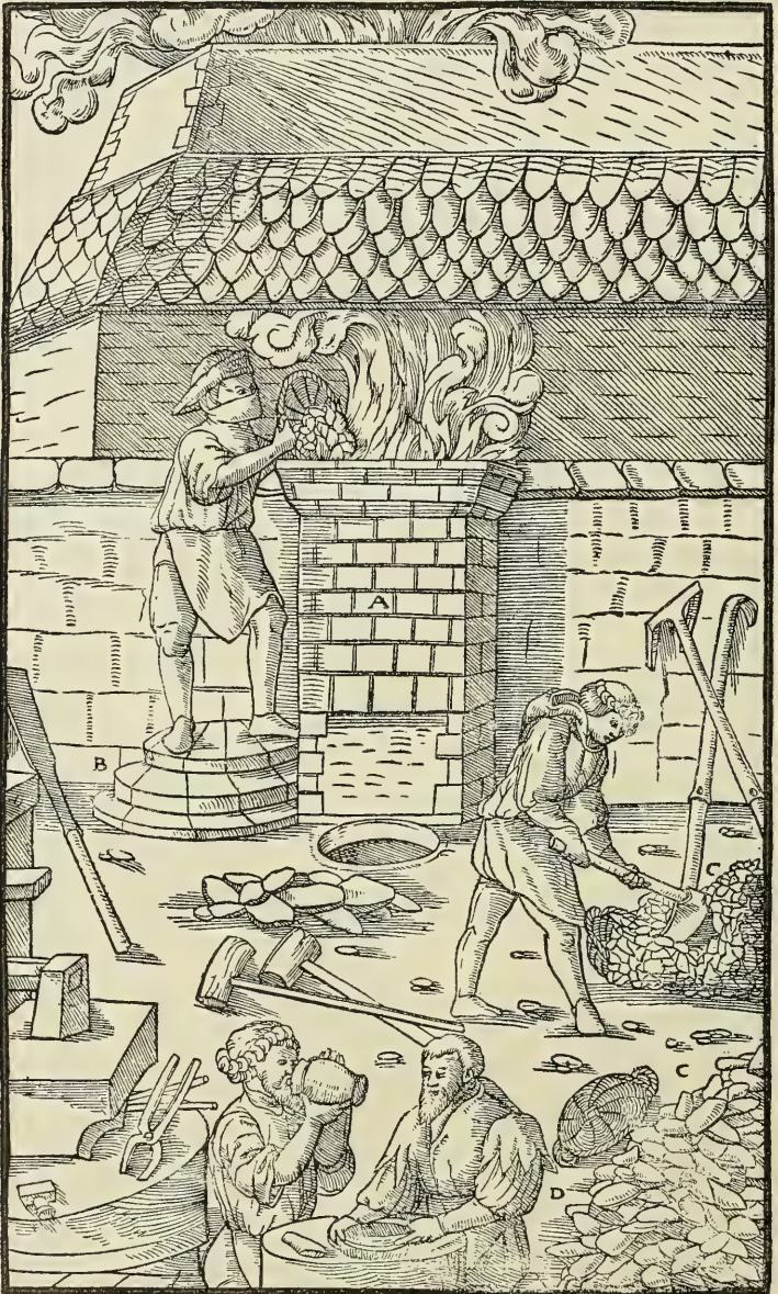
A—FURNACE. B—STAIRS. C—ORE. D—CHARCOAL.
