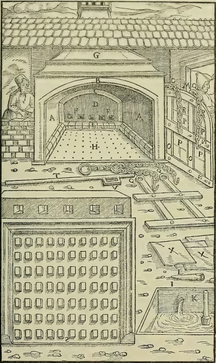
A—SIDE WALLS. B—FRONT ARCH. C—REAR ARCH. D—WALL IN THE REAR ARCH. E—INNER WALL. F—VENT HOLES. G—CHIMNEY. H—HEARTH. I—TANK. K—PIPE. L—PLUG. M—IRON DOOR. N—TRANSVERSE BARS. O—UPRIGHT BARS. P—PLATES. Q—RINGS OF THE BARS. R—CHAINS. S—ROWS OF BRICKS. T—BAR. V—ITS HAFT. X—COPPER BED-PLATES.
