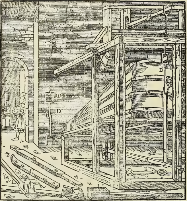
A—LEVER WHICH WHEN DEPRESSED BY MEANS OF A CAM COMPRESSES THE BELLOWS. B—SLOTS THROUGH THE POSTS. C—BAR. D—IRON IMPLEMENT WITH A RECTANGULAR LINK. E—IRON INSTRUMENT WITH ROUND RING. F—HANDLE OF BELLOWS. G—UPPER POST. H—UPPER LEVER. I—BOX WITH EQUAL SIDES. K—BOX NARROW AT THE BOTTOM. L—PEGS DRIVEN INTO THE UPPER LEVER.
