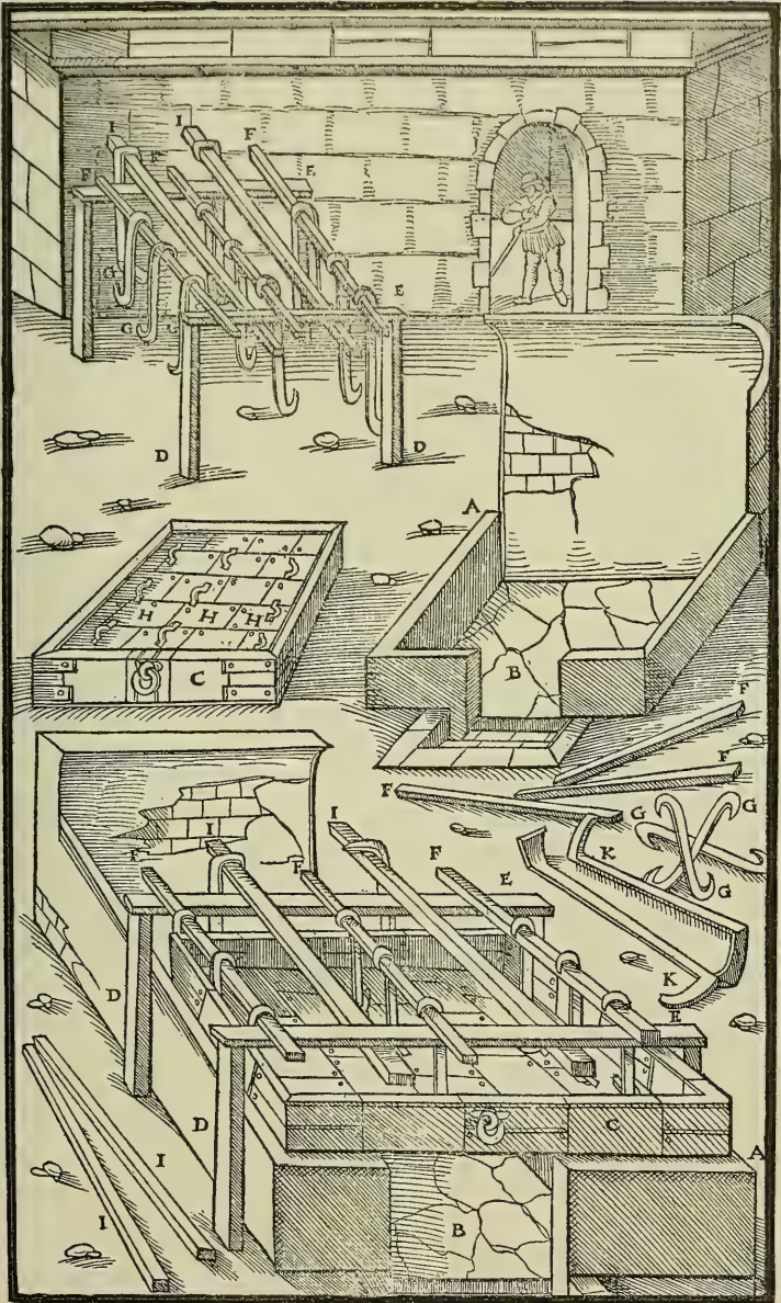
A—FIREPLACE. B—MOUTH OF FIREPLACE. C—CALDRON. D—POSTS SUNK INTO THE GROUND. E—CROSS-BEAMS. F—SHORTER BARS. G—IRON HOOKS. H—STAPLES. I—LONGER BARS. K—IRON ROD BENT TO SUPPORT THE CALDRON.
