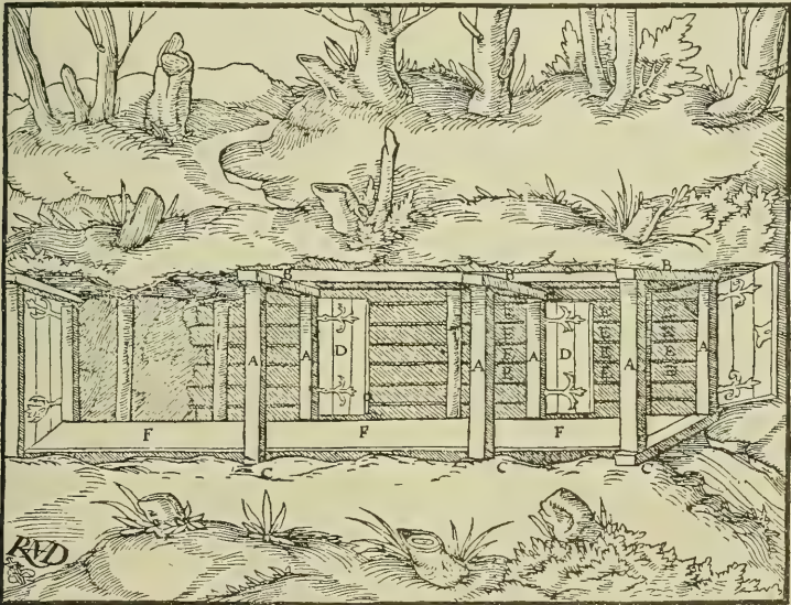
A—POSTS. B—CAPS. C—SILLS. D—DOORS. E—LAGGING. F—DRAINS.
