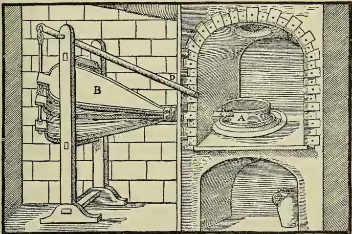
A—IRON HOOP. B—DOUBLE BELLOWS. C—ITS NOZZLE. D—LEVER.
