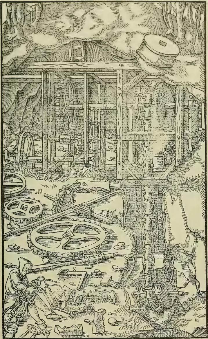
A—IRON FRAME. B—LOWEST AXLE. C—FLY-WHEEL. D—SMALLER DRUM MADE OF RUNDLES. E—SECOND AXLE. F—SMALLER TOOTHED WHEEL. G—LARGER DRUM MADE OF RUNDLES. H—UPPER AXLE. I—LARGER TOOTHED WHEEL. K—BEARINGS. I.—PILLOW. M—FRAMEWORK. N—OAK TIMBER O—SUPPORT OF IRON BEARING P—ROLLER. Q—UPPER DRUM. R—CLAMPS. S—CHAIN. T—LINKS. V—DIPPERS X—CRANK. Y—LOWER DRUM OR BALANCE WEIGHT.
