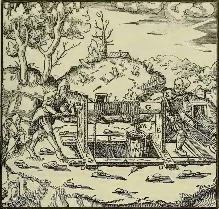
A—TIMBER PLACED IN FRONT OF THE SHAFT. B—TIMBER PLACED AT THE BACK OF THE SHAFT. C—POINTED STAKES. D—CROSS-TIMBERS. E—POSTS OR THICK PLANKS. F—IRON SOCKETS. G—BARREL. H—ENDS OF BARREL. I—PIECES OF WOOD. K—HANDLE. L—DRAWING-ROPE. M—ITS HOOK. N—BUCKET. O—BALE OF THE BUCKET.
