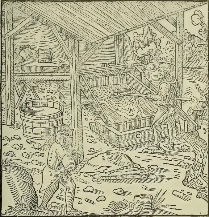
A—SHORT STRAKE. B—SMALL LAUNDER. C—TRANSVERSE LAUNDER. D—WOODEN SCRUBBER.
