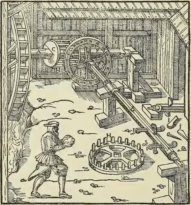
A—AXLE. B—WATER-WHEEL. C—DRUM COMPOSED OF RUNDLES. D—OTHER AXLE. E—TOOTHED WHEEL. F—ITS SPOKES. G—ITS SEGMENTS. H—ITS TEETH. I—CAMS OF THE AXLE.
