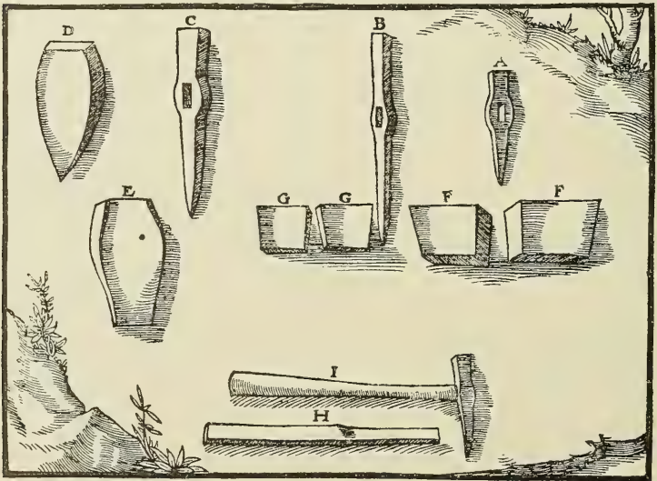
A—FIRST "IRON TOOL." B—SECOND. C—THIRD. D—FOURTH. 2 E—WEDGE. F—IRON BLOCK. G—IRON PLATE. H—WOODEN HANDLE. I—HANDLE INSERTED IN FIRST TOOL.
