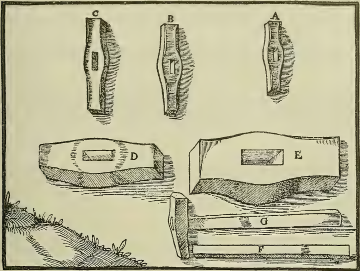
A—SMALLEST OF THE SMALLER HAMMERS. B—INTERMEDIATE. C—LARGEST. D—SMALL KIND OF THE LARGER HAMMER. E—LARGE KIND. F—WOODEN HANDLE. G—HANDLE FIXED IN THE SMALLEST HAMMER.
