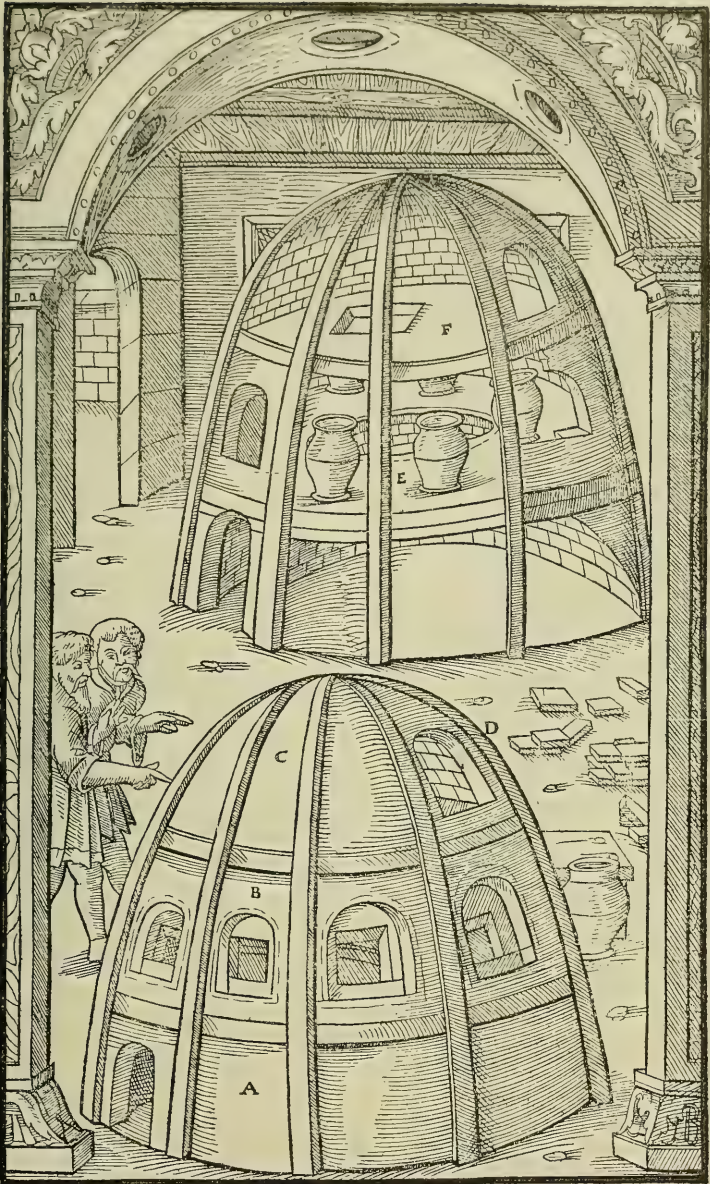
A—LOWER CHAMBER OF THE OTHER SECOND FURNACE. B—MIDDLE ONE. C—UPPER ONE. D—ITS OPENING. E—ROUND OPENING. F—RECTANGULAR OPENING.
