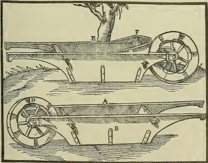
A—SMALL WHEELBARROW. B—LONG PLANKS THEREOF. C—END-BOARDS. D—SMALL WHEEL. E—LARGER BARROW. F—FRONT END-BOARD THEREOF.
