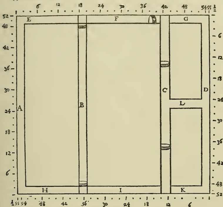
THE FOUR LONG WALLS: A—FIRST. B—SECOND. C—THIRD. D—FOURTH. THE SEVEN TRANSVERSE WALLS: E—FIRST. F—SECOND. G—THIRD. H—FOURTH. I—FIFTH. K—SIXTH. L—SEVENTH, OR MIDDLE.
