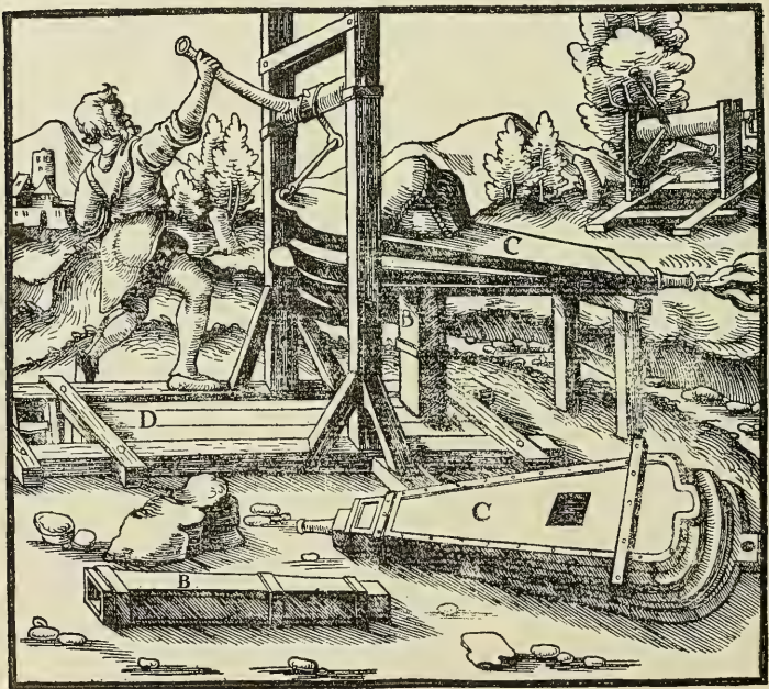
A—SMALLER PART OF SHAFT. B—SQUARE CONDUIT. C—BELLOW. D—LARGER PART OF SHAFT.
