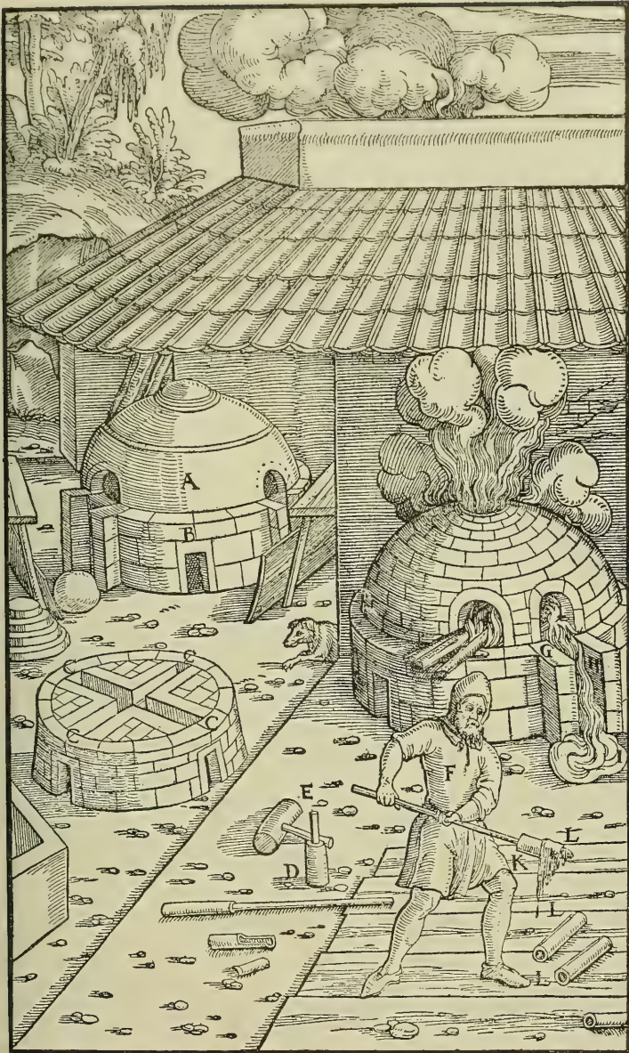
A—CHAMBER OF THE FURNACE. B—ITS BED. C—PASSAGES. D—RAMMER. E—MALLET. F—ARTIFICER MAKING TUBES FROM LITHARGE ACCORDING TO THE ROMAN METHOD. G—CHANNEL. H—LITHARGE. I—LOWER CRUCIBLE OR HEARTH. K—STICK. L—TUBES.
