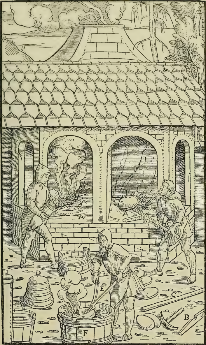
A—CRUCIBLE. B—BOARD. C—WEDGE-SHAPED BAR. D—CAKES OF COPPER MADE BY SEPARATING THEM WITH THE WEDGE-SHAPED BAR. E—TONGS. F—TUB.
