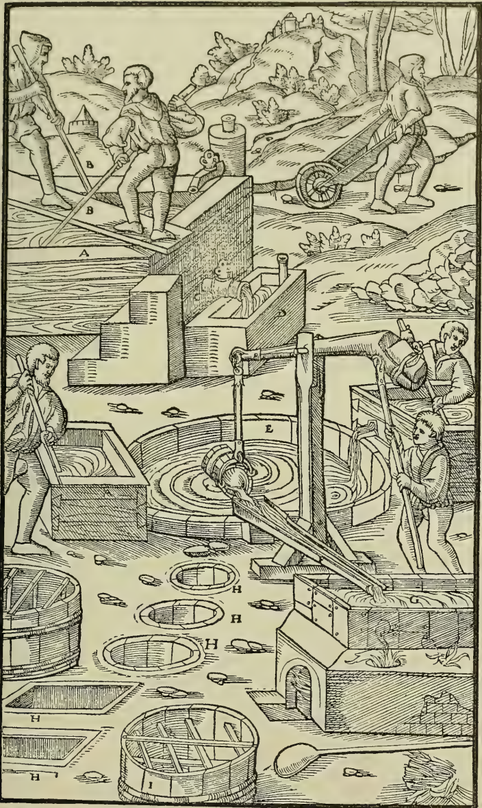
A—TANKS. B—STIRRING POLES. C—PLUG. D—TROUGH. E—RESERVOIR. F—LAUNDER. G—LEAD CALDRON. H—WOODEN TUBS SUNK INTO THE EARTH. I—VATS IN WHICH TWIGS ARE FIXED.
