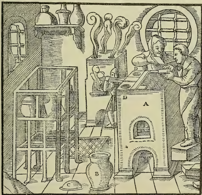
A—FURNACE. B—POT. C—LID. D—AIR-HOLES.
