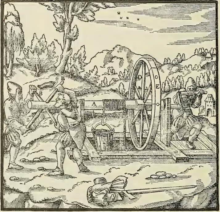
A—BARREL. B—STRAIGHT LEVERS. C—USUAL CRANK. D—SPOKES OF WHEEL. E—RIM OF THE SAME WHEEL.
