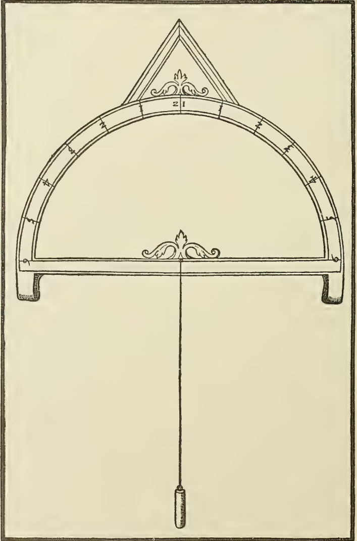
INDICATOR OF A SUSPENDED PLUMMET LEVEL.
