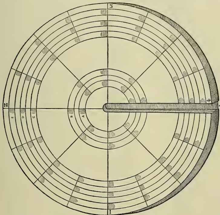
A, B, C, D, E—FIVE WAXED CIRCLES OF THE orbis. F—OPENING OF SAME. G—SCREW. H—PERFORATED IRON.
