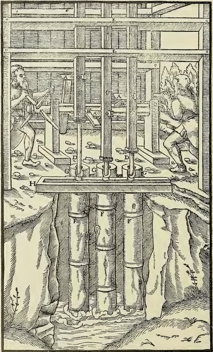
A—TAPPETS OF PISTON-RODS. B—CAMS OF THE BARREL. C—SQUARE UPPER PARTS OF PISTON-RODS. D—LOWER ROUNDED PARTS OF PISTON-RODS. E—CROSS-BEAMS. F—PIPES. G—APERTURES OF PIPES. H—TROUGH. (Fifth kind of pump—see p. 181).
