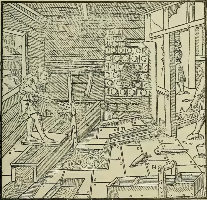
A—FIRST LAUNDRER. B—THREE-TOOTHED RAKE. C—SMALL SETTLING PIT. D—LARGE BUDDLE. E—BUDDLE RESEMBLING THE SIMPLE BUDDLE. F—SMALL ROLLER. G—BOARDS. H—THEIR HOLES. I—SHOVEL. K—BUILDING. L—STOVE. (THIS PICTURE DOES NOT ENTIRELY AGREE WITH THE TEXT).
