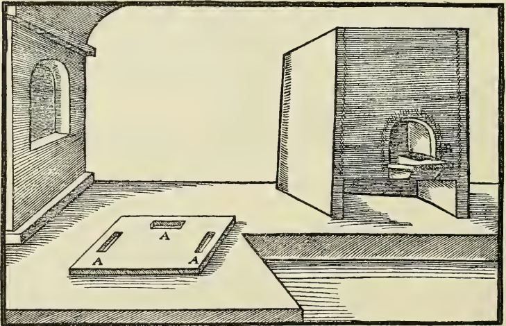
A—OPENINGS IN THE PLATE. B—PART OF PLATE WHICH PROJECTS BEYOND THE FURNACE.
