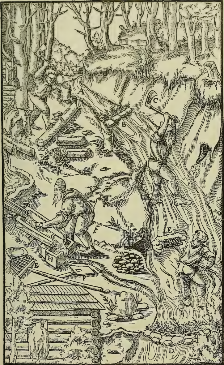
A—STREAM. B—DITCH. C—MATTOCK. D—PIECES OF TURF. E—SEVEN-PRONGED FORK. F—IRON SHOVEL. G—TROUGH. H—ANOTHER TROUGH. I—SMALL WOODEN TROWEL.
