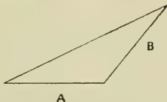
TRIANGLE HAVING AN OBTUSE ANGLE AND TWO EQUAL SIDES.
