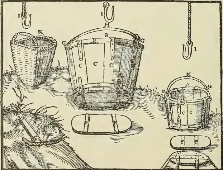
A—SMALL BUCKET. B—LARGE BUCKET. C—STAVES. D—IRON HOOPS. E—IRON STRAPS. F—IRON STRAPS ON THE BOTTOM. G—HAFTS. H—IRON BALE. I—HOOK OF DRAWING-ROPE. K—BASKET. L—HIDE BUCKET OR SACK.
