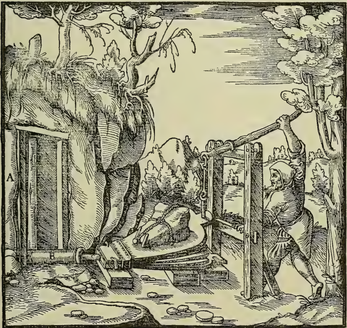
A—TUNNEL. B—PIPE. C—NOZZLE OF DOUBLE BELLOWS.
